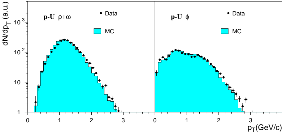
Fig. 9. Transverse momentum distributions measured in p-U collisions, compared with the expected sources, for the \rho + \omega (left) and \phi (right) mass windows
