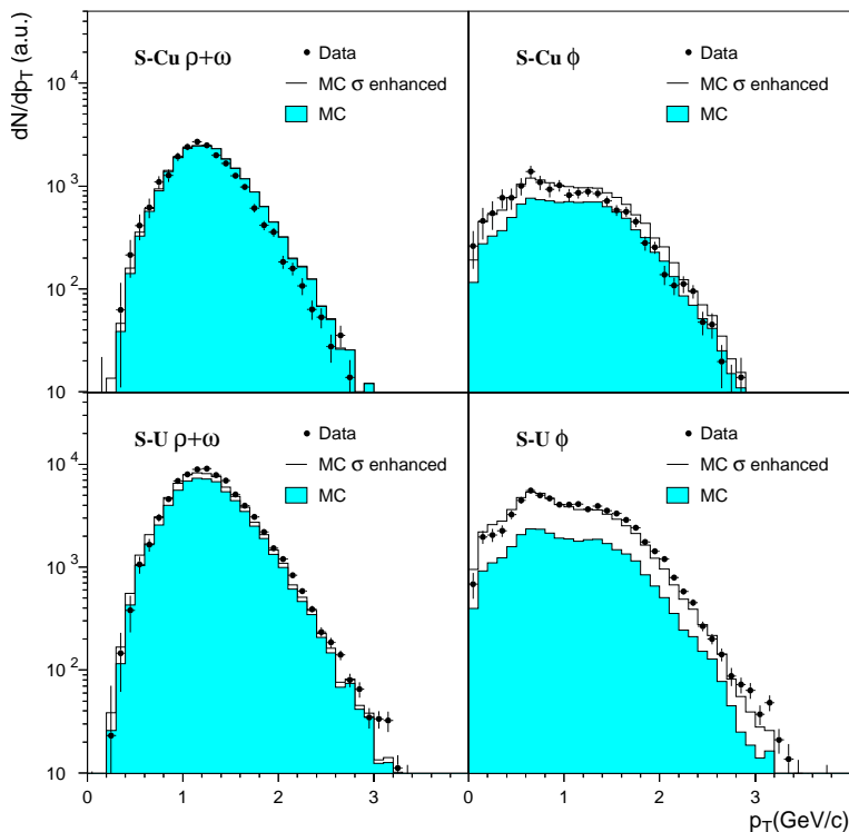
Fig. 13. Transverse momentum distributions measured in S-Cu (top) and S-U (bottom), compared with the expected sources, for the \rho+\omega (left) and \phi (right) mass windows
