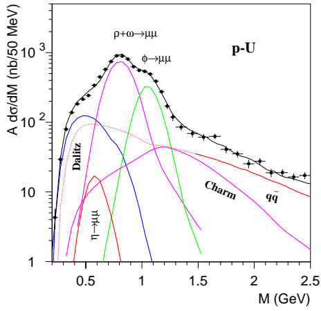
Fig. 5. Dimuon mass distribution measured in p-U collisions, compared to the new ‘cocktail’, including a roughly estimated contribution due to q\bar{q} annihilation
