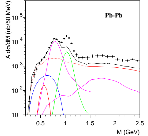
Fig. 11. Dimuon mass distribution measured in Pb-Pb collisions. The low mass region is considerably affected by the stronger m_T cut applied in this data set. The curves have the same meaning as in Fig. 5
