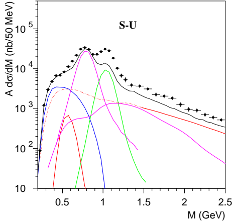
Fig. 10. Dimuon mass distribution measured in S-U collisions, compared to the (extended) cocktail of expected contributions. The curves have the same meaning as in Fig. 5
