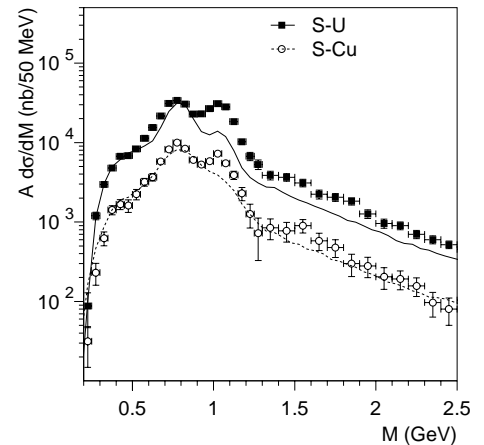
Fig. 12. Dimuon mass spectra measured in S-Cu and S-U collisions, compared, in each case, with the corresponding expected sources
