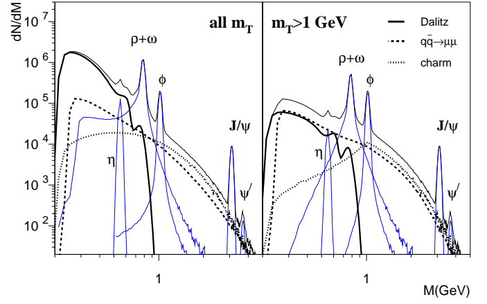
Fig. 7. Generated mass spectrum before (left) and after (right) selecting only events with m_T above 1 GeV
