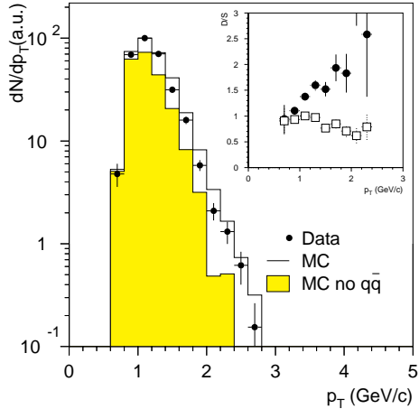
Fig. 6. Transverse momentum distributions measured in p-U, in the mass range 0.4 < M < 0.6 GeV, compared with the expected sources. The inset shows the ratio between the data and the expected sources with (open squares) and without (filled circles) the q\bar{q} annihilation process
