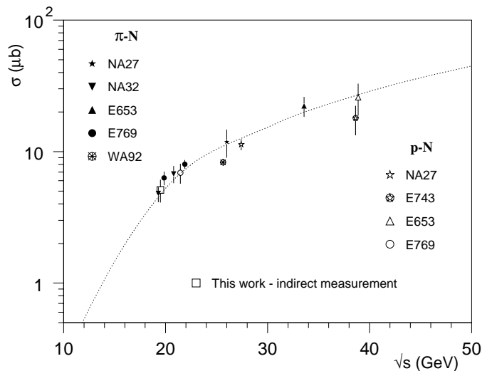
Fig. 2. Evolution of the c\bar{c} cross section with \sqrt{s}
