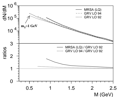
Fig. 8. Calculated mass spectrum for the q\bar{q} \rightarrow \mu\mu annihilation process, for three different sets of quark distribution functions. For the GRV LO 92 set we also show the calculation for m_T > 1 GeV dimuons. The lower panel shows the ratios relative to the estimation done with the GRV LO 92 set, which has the lowest Q_{\min}^2
