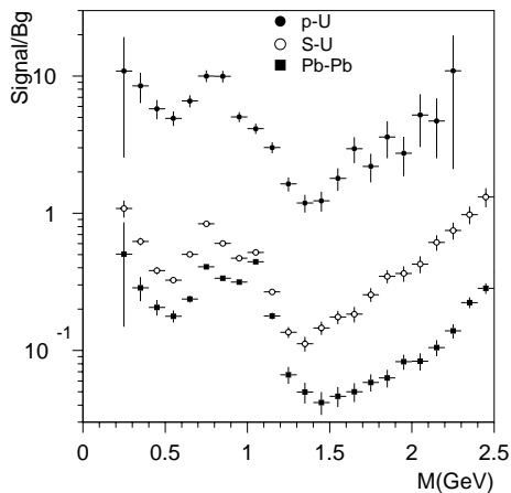
Fig. 1. Signal over background ratio as a function of the dimuon mass for p-U, S-U and Pb-Pb collisions
