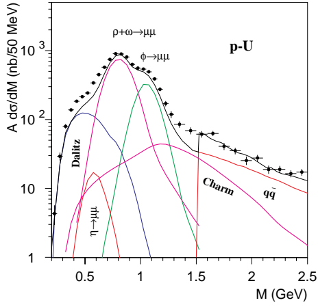
Fig. 4. Dimuon mass distribution measured in p-U collisions, compared to the superposition of expected processes
